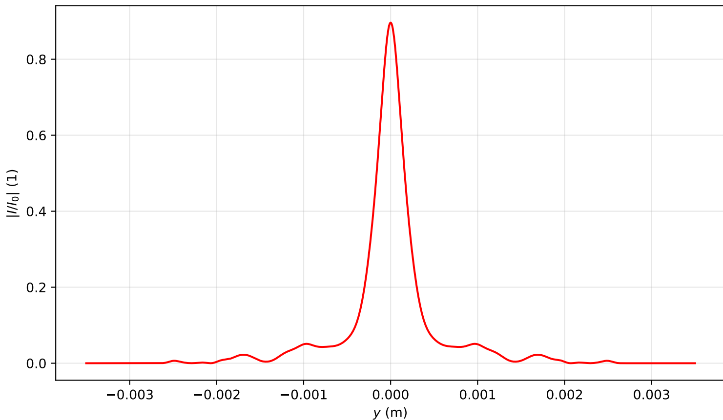
Intensity profile I(x=0, y, z=2.866)/I_0 , P_{in}=4.5P_{cr} , artificial time
